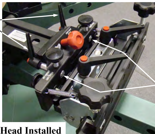
Print Head Mounting Bolts
